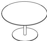
ODETTE LOW TABLE Top SC-04 Ø:100 Base SC-124 H:42
