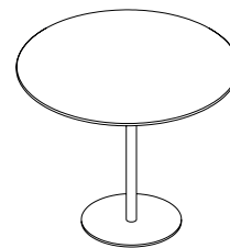
ODETTA DINING TABLE Top SC-11 Ø:126 Base SC-126 H:72 Tops available in Metal and Laminate.
