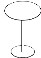
ODETTE BAR TABLE Top SC-03 Ø:75 Base SC-117 H:110
