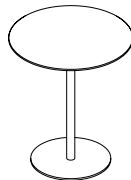
ODETTE BAR TABLE Top SC-03 Ø:75 Base SC-116 H:100
