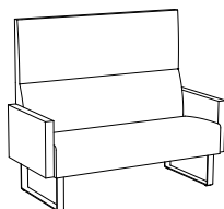
SA610/SA620/SA630 H 1230 SH 450 B 680/1430/1830 D 630
