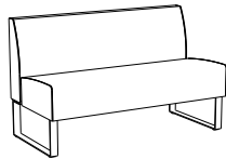
SA610/SA620/SA630 H 795 SH 450 B 560/1310/1710 D 630
