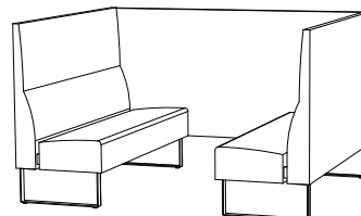
SA610/SA620/SA630 H 1230 SH 450 B 680/1430/1830 D 630
