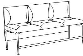
SA830 rak koppling (14) H 1030 SH 630 B 1910 D 650
