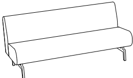
SA410 3-sits, bengavel x2 H 800/830 SH 440/470 B 1800 D 700
