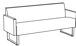
SA610/SA620/SA630 H 795 SH 450 B 680/1430/1830 D 630
