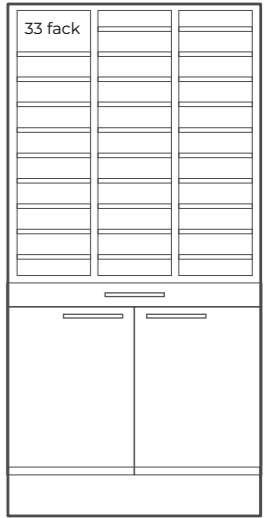
PS9/19 1932x910x372
