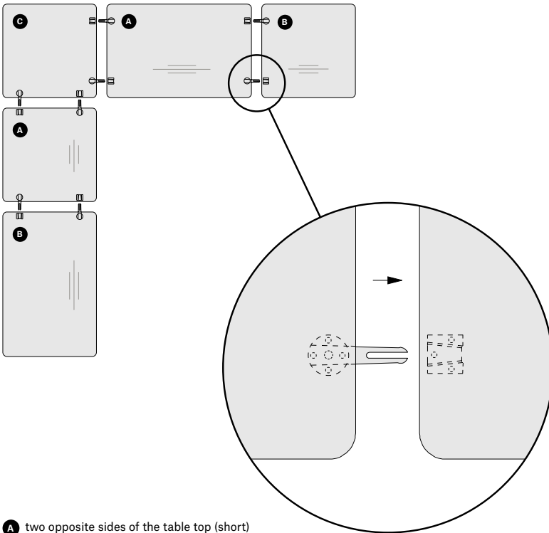
Configuration of connecting hardware on table top
