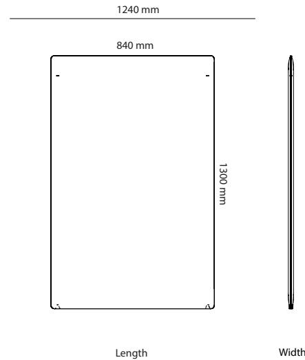
Wall screen
